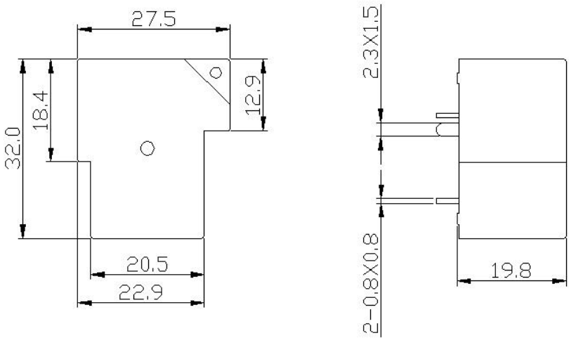
安装孔尺寸图/ Mounting dimension(bottom view)
