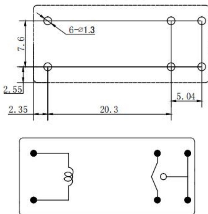
安装孔尺寸图/ Mounting dimension(bottom view)
